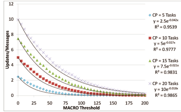
Figure 6: The effect of Slack with selected critical paths on a low variance Gaussian
