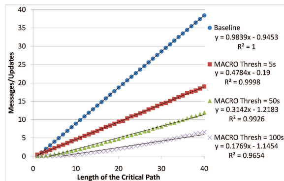
Figure 4: The effect of critical path length with selected thresholds with a low variance Gaussian
