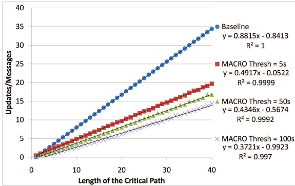
Figure 5: The effect of critical path length with selected thresholds with a high variance Gaussian
