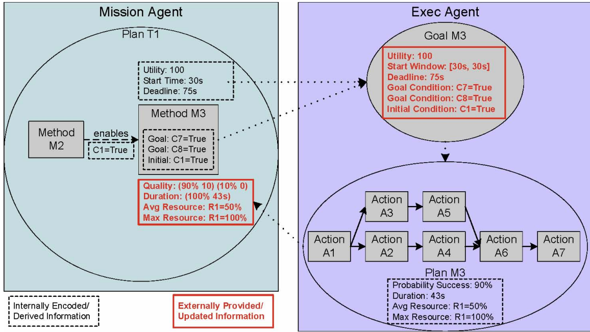
Figure 2: Planning/Scheduling Translation in MACRO
