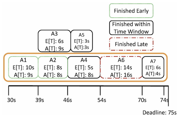
Figure 3: A Resource-level Plan (Critical Path Highlighted)
