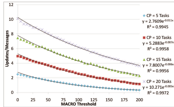
Figure 7: The effect of Slack with selected critical paths on a high variance Gaussian
