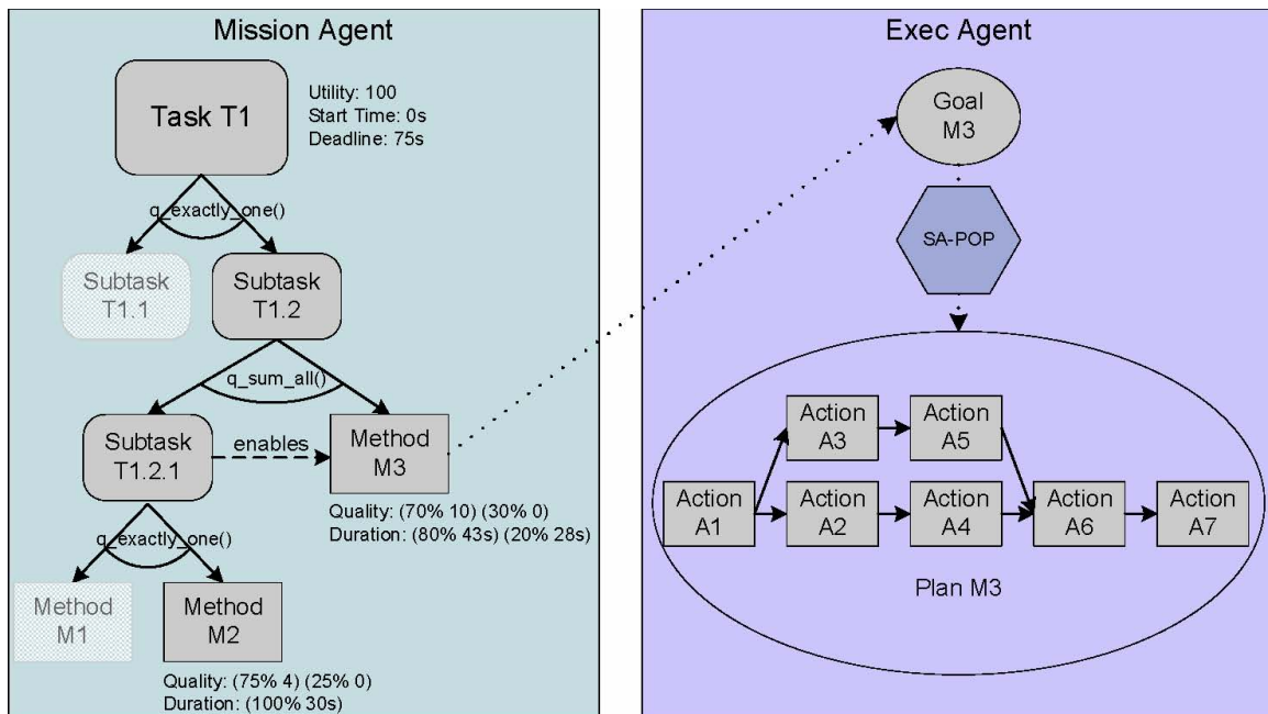
Figure 1: Planning/Scheduling Representations in MACRO
